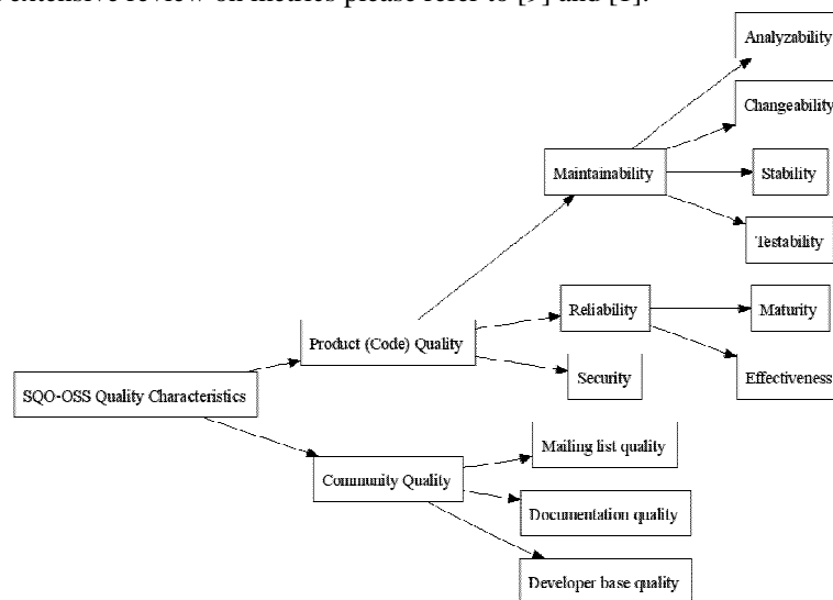
Fig. 1 The SQO-OSS quality model.
