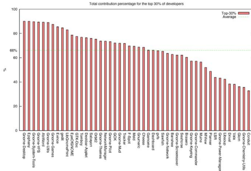
Figure 35. Total contribution from the top 30% of developers for various projects
