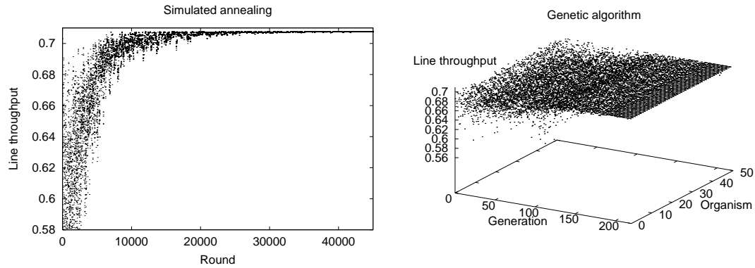
Figure 2: Stochastic method operation comparison
