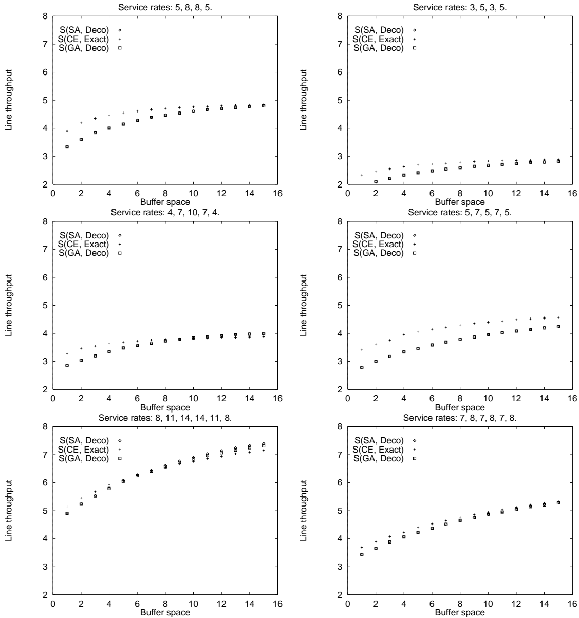
Figure 4: Simulated annealing S(SA, Deco) and genetic algorithms S(GA, Deco) with decomposition evaluation versus complete enumerated Markovian S(CE, Exact) throughputs for unbalanced lines with 4–6 stations.
